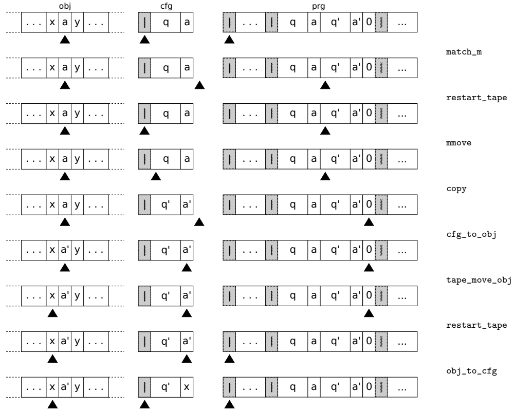
Figure 2: Sample execution of unistep .
