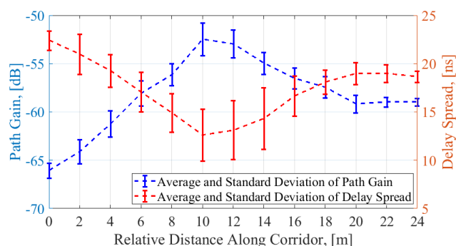
FIGURE 7. Average and standard deviation of the path gain and delay spread during continuous UAV flights.
