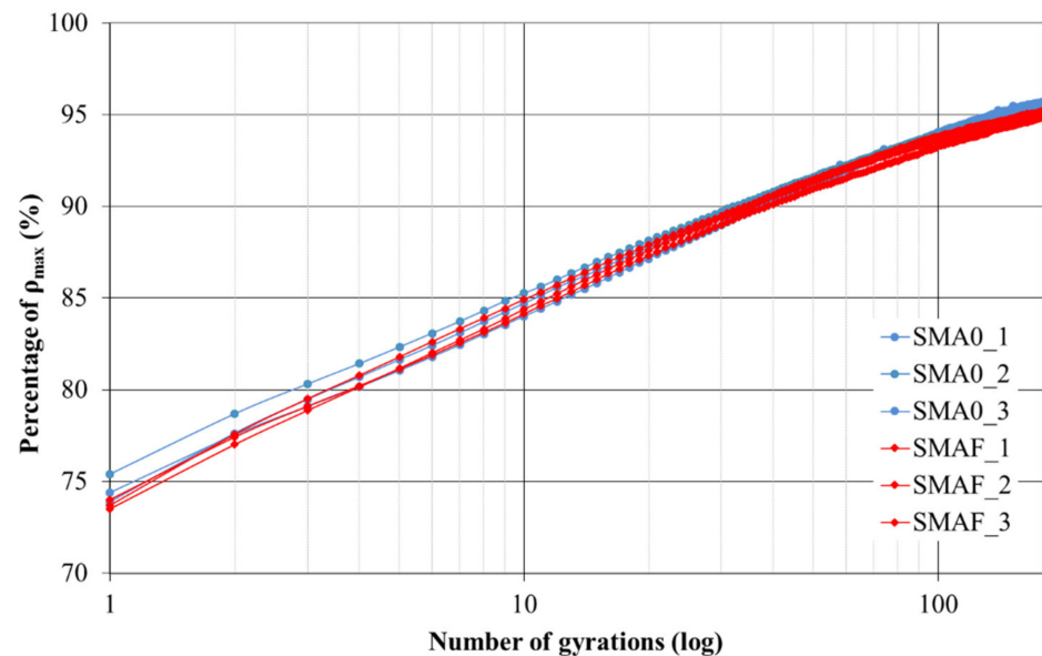
Figure 3. Bituminous mixtures gyratory compaction curves.
