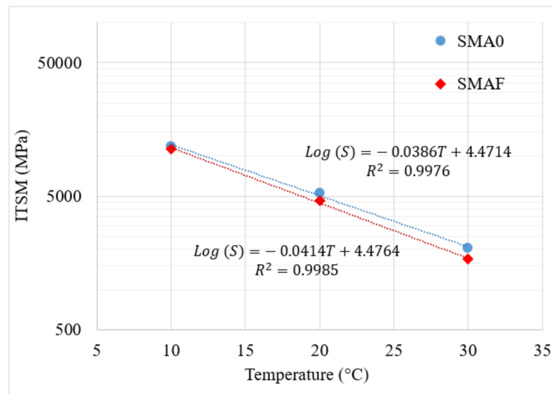
Figure 4. ITSM average results and temperature sensitivity.
