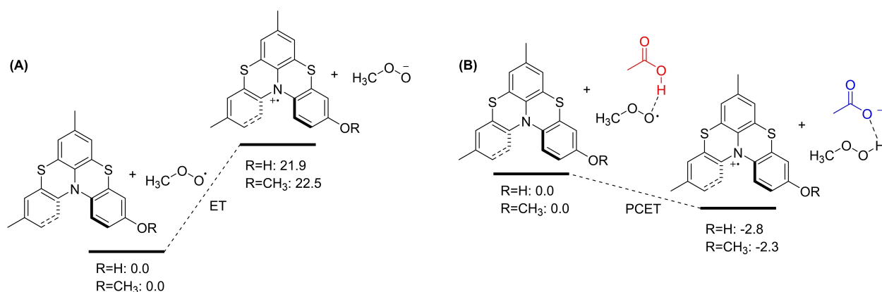
Figure 7. DFT-computed free energy for the electron transfer from helicenes 2 ( R=CH_3 ) and 5 ( R=H ) toward CH_3OO^\bullet radical in the absence (A) or in the presence (B) of acetic acid. Proton transfer from CH_3COOH to CH_3OO^- is barrierless and occurs during the geometry optimization. Calculations performed at the B3LYP/6-311+g(d,p) level with implicit MeCN solvent and one explicit MeCN molecule when R=H .
