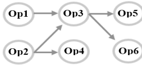
Fig. 2. Precedence graph
