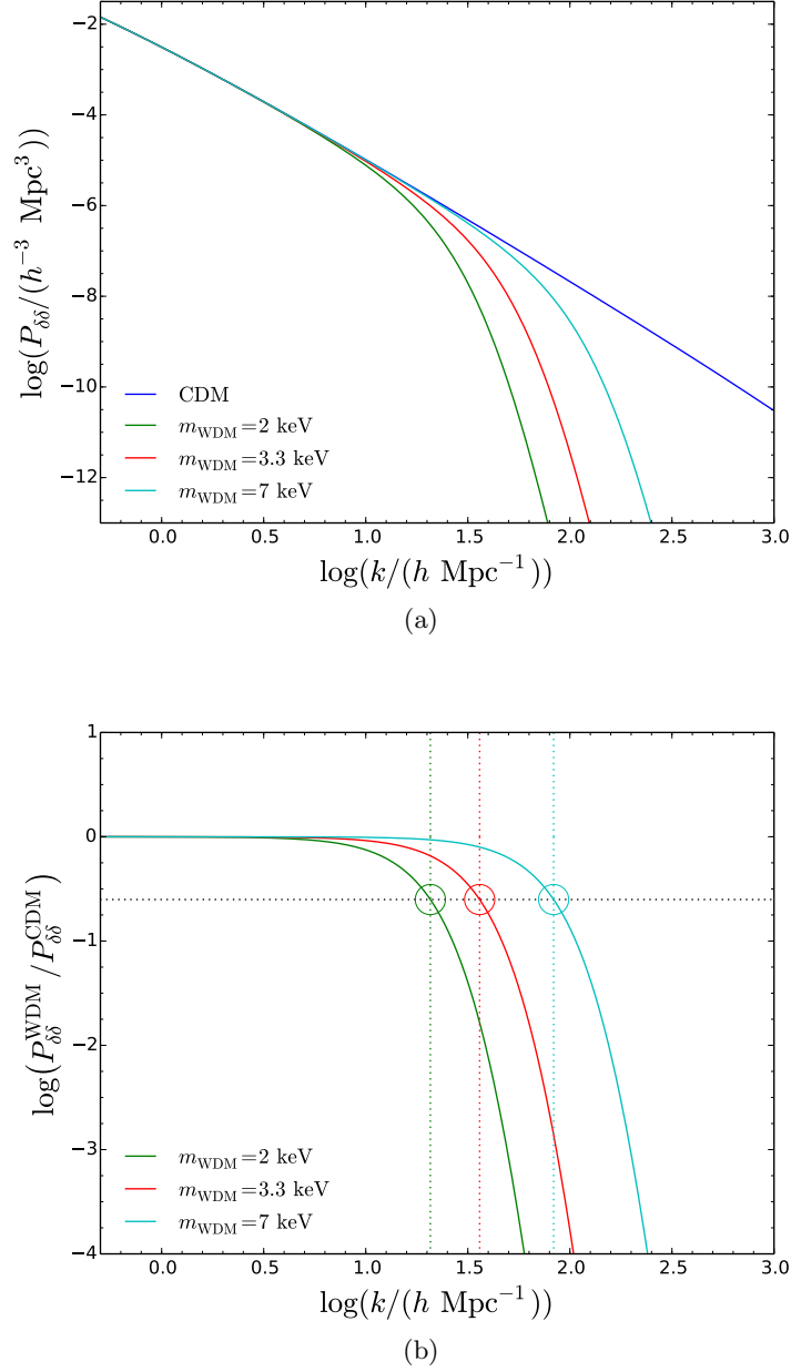
Figure 1. (a) Linear theory matter power spectra at redshift z = 199 for CDM and three WDM models with masses m_{\text{WDM}} = 2, 3.3, 7 \text{ keV} as labelled. (b) Squared transfer functions T^2(k) \equiv P^{\text{WDM}}_{\delta\delta}/P^{\text{CDM}}_{\delta\delta}(k) for the three warm candidates. The dotted black horizontal line represents the scale at which the transfer function is suppressed by a factor of two. The intersection between the transfer function and the horizontal line defines the half-mode wavenumber k_{\text{hm}} . The WDM spectra are generated using the parametrisation in eq. (2.3).
