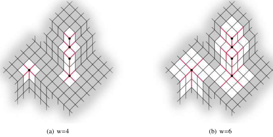
Figure 9: Mesh containing several extraordinary vertices. The regular regions are highlighted in grey for support width w = 4 and w = 6 .
