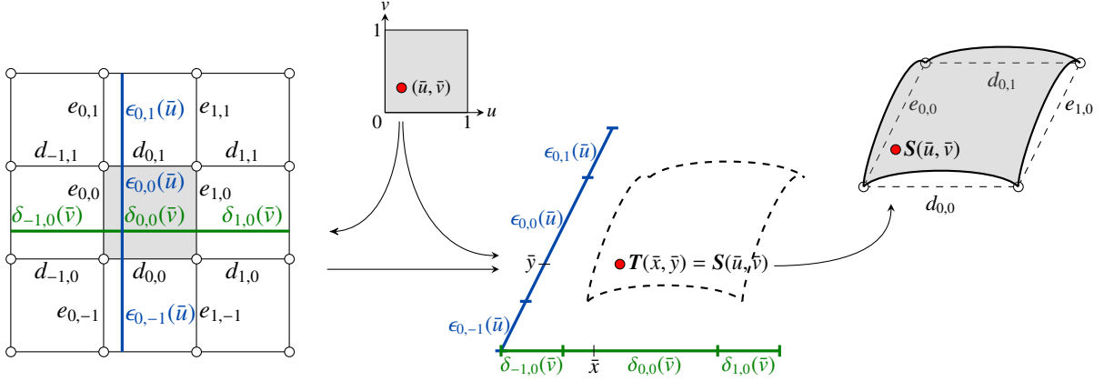
Figure 4: Construction of an augmented patch in the case of support width w = 4 .
