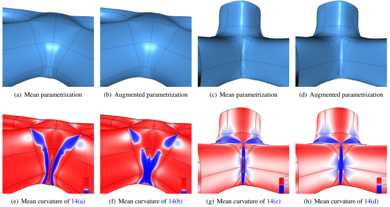
Figure 14: Zoom of the surfaces obtained from the meshes in Figure 13 with augmented and mean parametrization.
