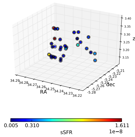
Fig. B.17. Same as Fig. B.1 for the overdensity detected at z = 3.27 in the UDS.
