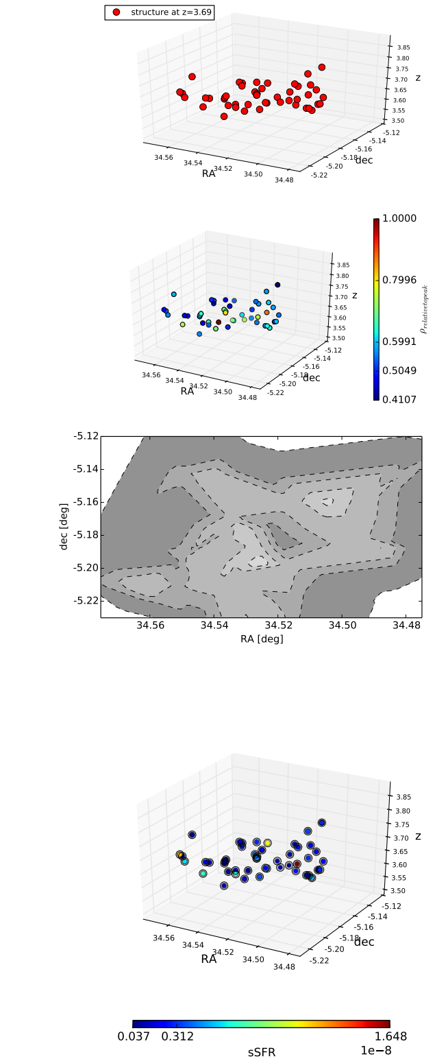
Fig. B.21. Same as Fig. B.1 for the overdensity detected at z = 3.69 in the UDS.
