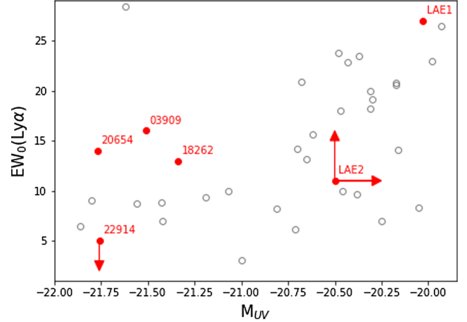
Fig. 4. EW(Ly\alpha) vs. M_{UV} for the six LSS-member galaxies of Table 1 (red filled circle). For comparison, we also plot the same properties for a large sample of high- z galaxies, presented by De Barros et al. (2017; gray empty circles).
