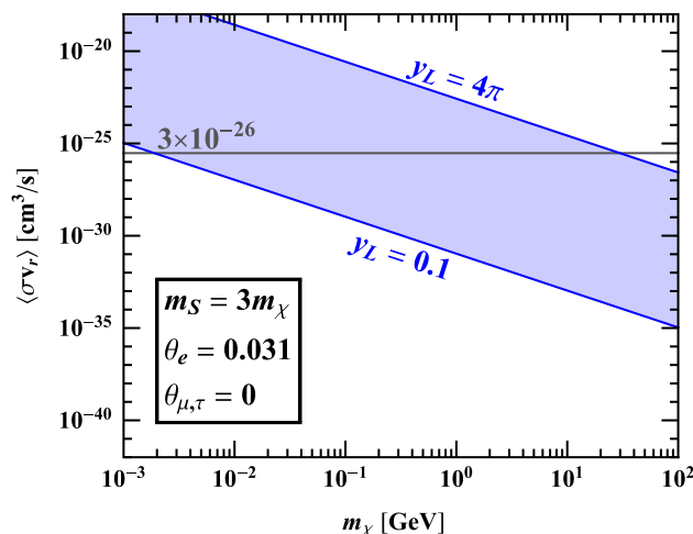
Fig. 2 Thermally averaged annihilation cross section multiplied by the relative velocity for \chi\bar{\chi} \rightarrow \nu\bar{\nu} . We have fixed m_S = 3m_\chi , \theta_e = 0.031 , \theta_\mu = \theta_\tau = 0 , and varied y_L between 0.1 and 4\pi
