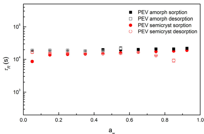
Figure 10. Plot of time of relaxation ( \tau_R ) from the BH model for water vapor at 20 °C in amorphous and semicrystalline PEV for sorption and desorption (two replicates for each point).
