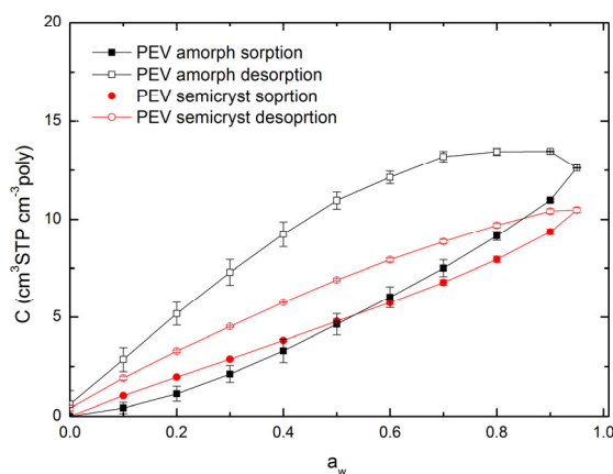
Figure 7. Sorption hysteresis at 20 °C for amorphous and semicrystalline PEV (two replicates for each point). Lines are drawn to aid the eye and do not represent model fits.
