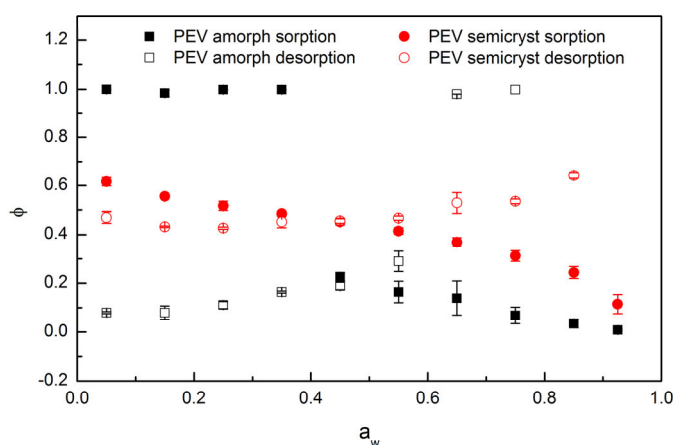
Figure 9. Plot of \phi from the BH model for water vapor at 20 °C in amorphous and semicrystalline PEV for sorption and desorption (two replicates for each point).
