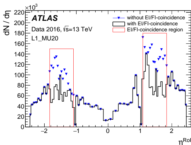
Figure 3. Pseudorapidity distributions of the L1 muon trigger with a p_T threshold of 20 GeV (L1_MU20) and the rate reduction due to requiring a coincidence with TGCs consisting of Endcap Inner (EI) and Forward Inner (FI) chambers are shown, using events taken by a lower-threshold L1 trigger (L1_MU11) in 2016. The \eta^{\text{RoI}} distribution after the inclusion of the EI/FI-coincidence is shown as a solid black line. The \eta^{\text{RoI}} distribution before the inclusion of the EI/FI-coincidence is also shown as a reference (blue triangles) to examine the reduction of the L1_MU20 trigger rate at 1.05 < |\eta| < 1.8 , which is highlighted by the red rectangles. No coincidence was required for |\eta| \sim 1.5 because the FI chambers in this region were inactive, which explains the lack of rate reduction. Moreover, the coincidence around |\eta| \sim 1.2 was intentionally not applied, to allow commissioning of a coincidence with the TileCal.
