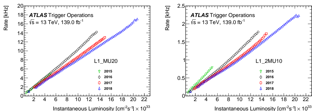
Figure 10. L1 trigger rates as a function of the instantaneous luminosity for the lowest unprecaled single-muon and dimuon triggers, L1_MU20 (left) and L1_2MU10 (right), in different years in Run 2.
