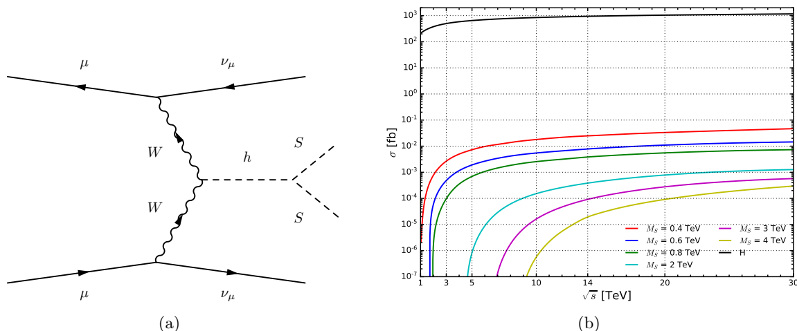
Figure 9. (a) Diagrammatic representation of SS pair production through W^+W^- fusion in a scalar singlet extension of the SM. (b) SS pair production cross section [fb] via EW VBF in \mu^+\mu^- collisions as a function of collider energy \sqrt{s} [TeV] for representative coupling inputs. Also shown for comparison is the H production process via EW VBF (black curve) in the SM.
