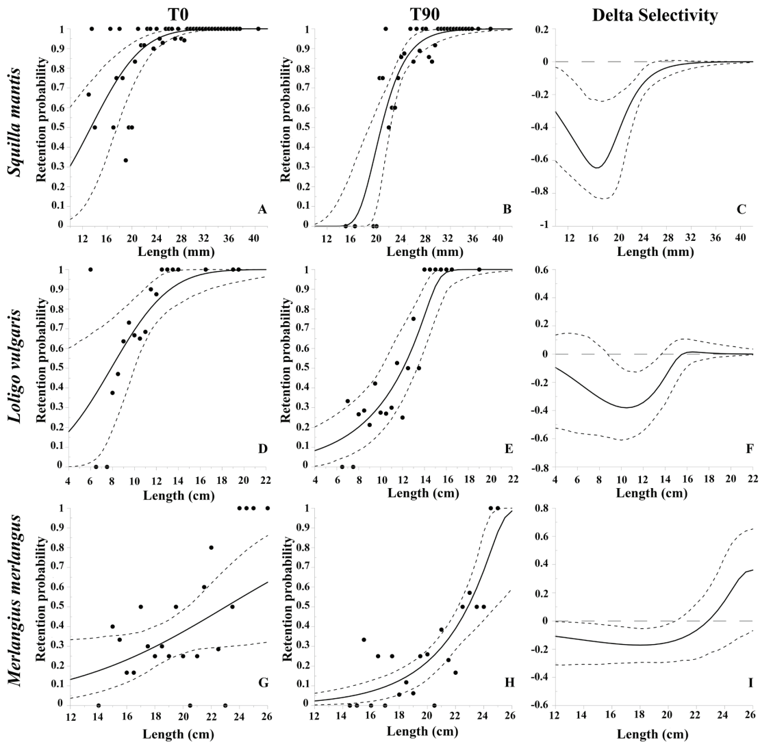
Fig. 3: Selectivity diagrams for Squilla mantis (A, B, C), Loligo vulgaris (D, E, F) and Merlangius merlangus (G, H, I). The first two columns show the size selectivity curves (full lines) with confidence intervals (dashed lines) and the experimental retention data (black dots) obtained with the T0 (A, D, G) and the T90 (B, E, H) codends. The right column shows the delta selectivity curve (full line) with confidence intervals (dashed lines) representing the differences between the curves of the two codends for each species.
