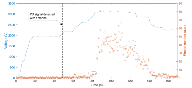
Fig. 7. PD activity detection in a motor by means of the optic sensor, using 50 Hz AC voltage. The latter is expressed in peak-to-peak.
