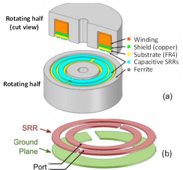
FIGURE 16. View of the wireless power and information transfer device: (a) cut view of the complete sub-system; (b) detail of the grounded SRR adopted for information transfer [51].
