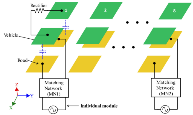
FIGURE 2. Schematic representation of capacitive WPT system made of repetitive Tx modules (yellow trapezoids) and the Rx plates (green trapezoids) [33].
