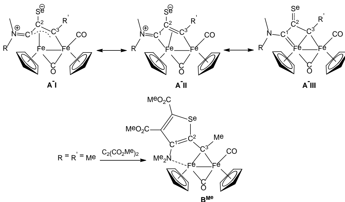
Scheme 1. Resonance forms representing a bridging Se-derivatized \text{C}_3 ligand ( A-I : allylidene; A-II : vinyliminium; A-III : bis-alkylidene), and alkyne cycloaddition to form a \mu -alkylidene-selenophene derivative ( B Me ). 26 R = Me or Xyl = 2,6- \text{C}_6\text{H}_3\text{Me}_2 ; R' = alkyl, aryl or \text{CO}_2\text{Me} .
