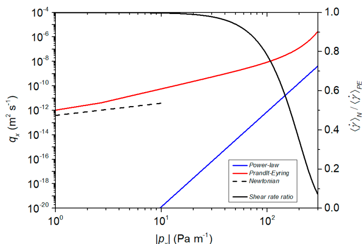
Figure 8. Plot of flow rate vs. pressure gradient; the red solid line represents the Prandtl–Eyring model ( A = 0.003465 Pa and B = 0.0231 s ^{-1} ), the blue solid line represents the power-law model ( \bar{\mu} = 0.0175 Pa \times s ^n and n = 0.13 ), and the black dashed line represents the Newtonian model ( \mu = A/B = 0.15 Pa \times s). The plot of shear rate ratio \langle \dot{\gamma} \rangle_N / \langle \dot{\gamma} \rangle_{PE} vs. pressure gradient is illustrated by the black solid line.
