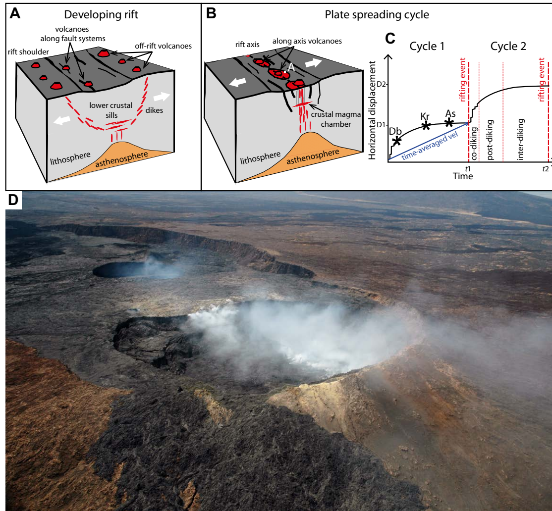
Figure 1. Rift zone illustration. (A) Thinning of the continental lithosphere causing dikes to ascend diagonally away from rift center, creating volcanoes off rift. Earlier volcanoes created during rift initiation along fault systems are also shown. (B) Volcanic segments during plate spreading. (C) The rift-perpendicular horizontal motion of point A, near the rift axis, at different phases during the plate spreading cycle. D is the total displacement for each full cycle and t , the time of a cycle, which is \sim 10^2\text{--}10^3 yr based on data from Iceland. The amount of opening varies in different segments; a widening of 4–5 m occurred during the codiking period in Krafla, Iceland. Existing volcanic segments currently undergoing different phases of the cycle: Db—Dabbahu rift (Afar), Kr—Krafla rift (Iceland), As—Askja rift (Iceland). (D) The Erta Ale volcano (Ethiopia), where the 0.7x1.6 km summit crater holds two lava lakes.
