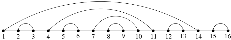
FIGURE 2.2. A planar matching
