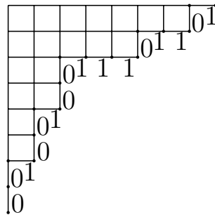
FIGURE 2.3. A Ferrers diagram and its d -code
