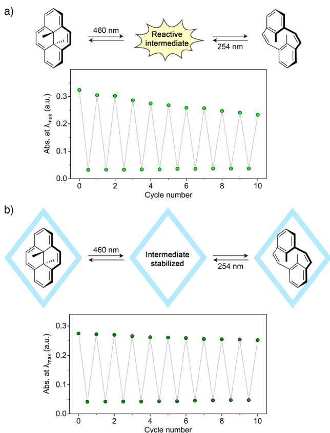
Figure 7. (a) Poor fatigue resistance of free DHP in pentane solution over 10 switching cycles. (b) Improved fatigue resistance of DHP@C1 in water over 10 switching cycles. Deoxygenated solvents were used. In each cycle, the samples were exposed to 10 min of blue light ( \lambda = 460 nm) followed by 10 min of UV light ( \lambda = 254 nm).
