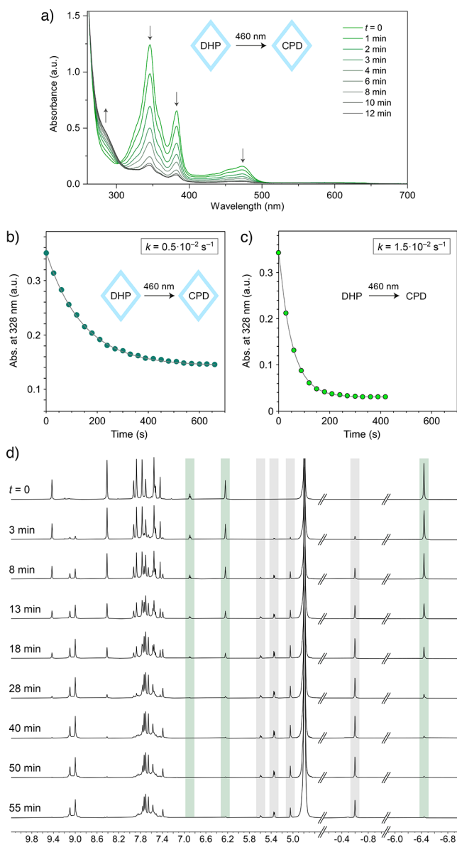
Figure 4. (a) A series of UV/vis absorption spectra of DHPc1 accompanying irradiation with 460 nm light. (b) Kinetics of photoisomerization of DHP to CPD in water at 20 °C. (c) Kinetics of photoisomerization of DHP to CPD in acetonitrile at 20 °C. Experiments in (b) and (c) were performed with the same irradiation setup ( \lambda_{\text{irr}} = 460 \text{ nm} ) under a pseudo-first-order regime ( A_{460} \ll 1 ). 47 Both time profiles were fitted with a first-order model (gray lines), and apparent first-order rate constants are reported. (d) Partial ^1\text{H} NMR spectra (400 MHz, \text{D}_2\text{O} ) of DHPc1 recorded after different times of irradiation with 460 nm light. Signals highlighted in green and gray originate from DHP and CPD, respectively.
