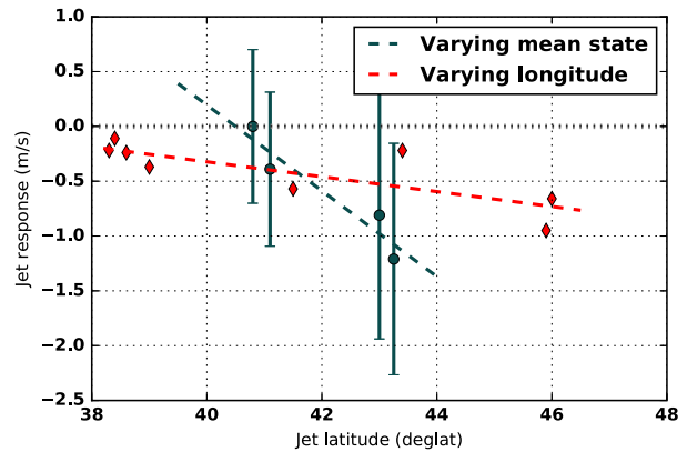
FIG. 11. Red diamonds indicates the response of the zonal wind at 300 hPa ( 50^{\circ} – 80^{\circ} N) in series N plotted vs the climatological jet latitude averaged in the sector where the heating is applied. Black circles show the response of the zonal wind at 300 hPa ( 50^{\circ} – 80^{\circ} N) for experiments in series Z (Z0, Za, Zb, Zc) plotted vs the climatological jet latitude averaged zonally. The response is averaged between month 1 and month 12. Bars indicate where the response is not statistically significant at 95% confidence interval according to a t test. Dashed lines are linear fits.
