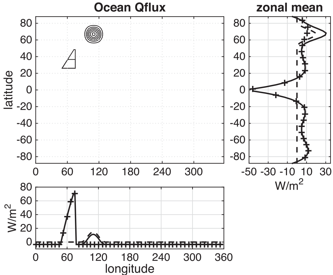
FIG. 2. Illustration of the experimental setup. (top left) The Q flux used for experiment N109. (bottom left) The meridional average and (right) the zonal average of the Q_{\text{TOTAL}} (solid line), Q_{\text{Track}} (crosses), and Q_h (dashed line). Note that the zonal mean of Q_{\text{Track}} is equal to that of Q_{\text{Sym}} .
