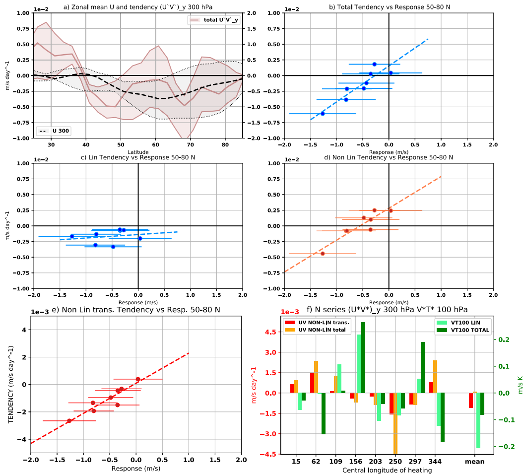
FIG. 9. (a) Median, maximum, and minimum values in N series of the total momentum flux convergence anomaly (solid; m s^{-1} day^{-1} ; left axis) and of anomalous zonal wind (dashed; m s^{-1} ; right axis) at 300 hPa and zonally averaged. Anomalies are computed by averaging between months 4 and 12 and subtracting the climatology of CONTROL0. Note that in these experiments the central latitude of the heating is fixed. (b) Relationship between the momentum flux convergence shown in (a) averaged between 50° and 80°N and the response of the zonal-mean zonal wind at 300 hPa defined as in (a). (c) As in (b), but for the linear component of the momentum flux convergence. (d),(e) As in (b), but for the nonlinear component and for the nonlinear component of transient synoptic eddies, respectively. See appendix for exact definition of linear and nonlinear components. Bars indicate the interval where the response is not statistically significant at 95% confidence according to a Student's t test. (f) Summary of nonlinear momentum convergence (total and transient synoptic eddies in yellow and red, respectively) at 300 hPa and total and linear eddy heat flux at 100 hPa (dark green and light green, respectively). Values are deviations from the multi-experiment mean that is displayed toward the right side of (f). Note the different y axes.
