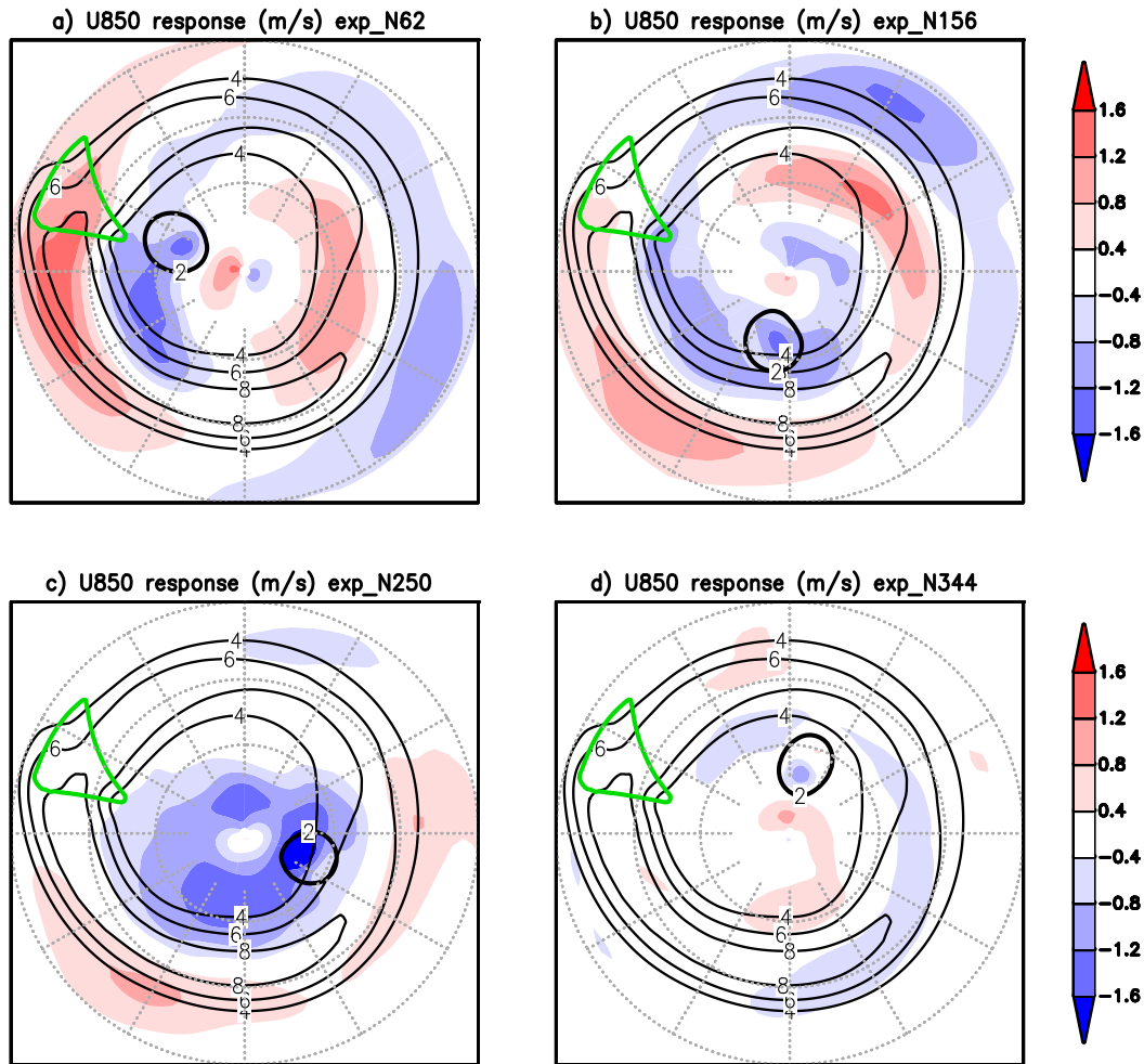
FIG. 5. Climatological zonal wind at 850 hPa in CONTROL0 (thin black contours) and anomalous zonal wind at 850 hPa (colors; \text{m s}^{-1} ) averaged from month 4 to month 12 for experiments (a) N62, (b) N156, (c) N250, and (d) N344. A thick black contour drawn at 2 K indicates anomalous temperature at 850 hPa. A green contour indicates the position of the storm-track triangle.
