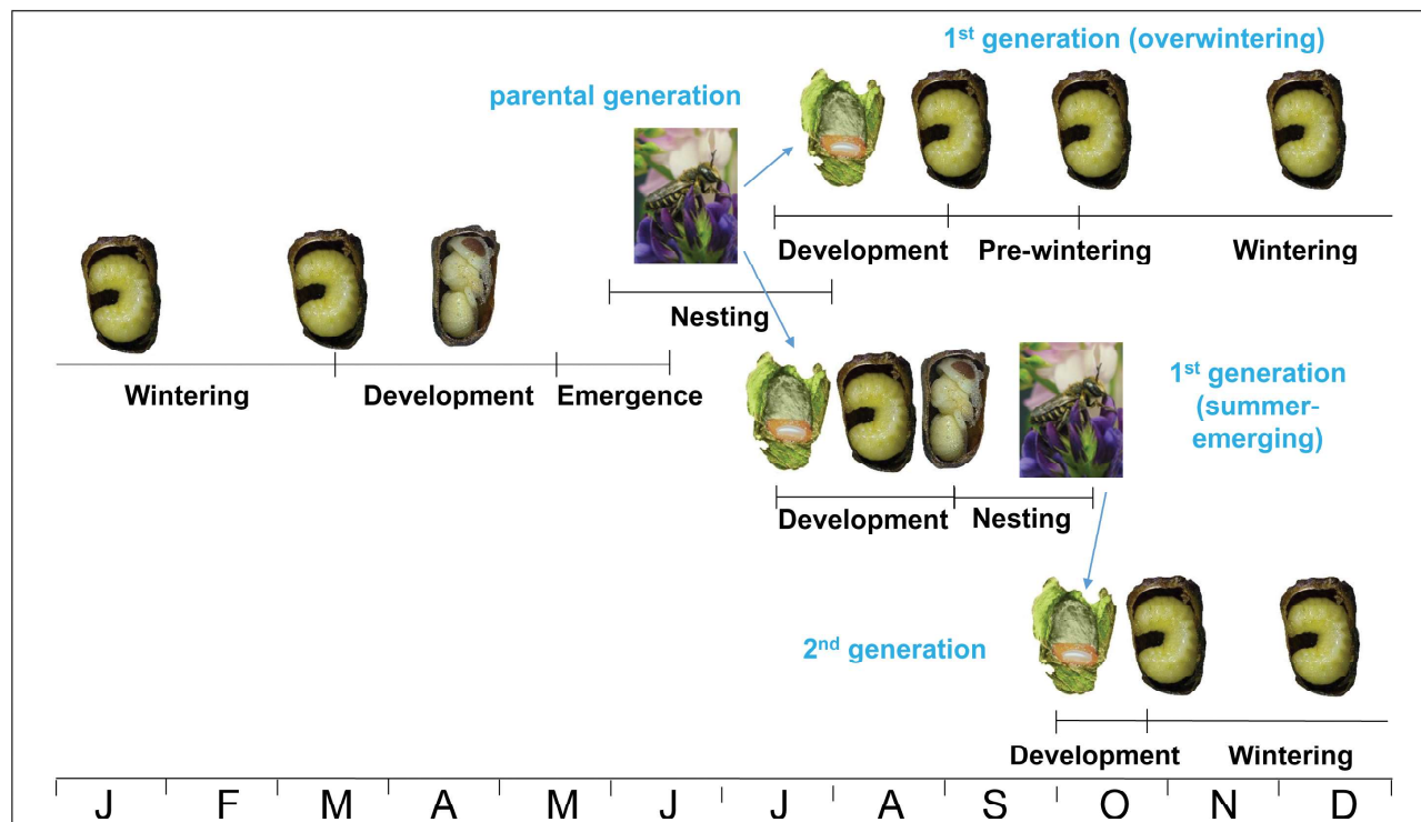
Fig. 4. Life cycle of Megachile rotundata . Photo credits: egg (Bill Nye), prepupa (Alan Anderson), pupa (Alan Anderson), adult (Theresa Pitts-Singer).
