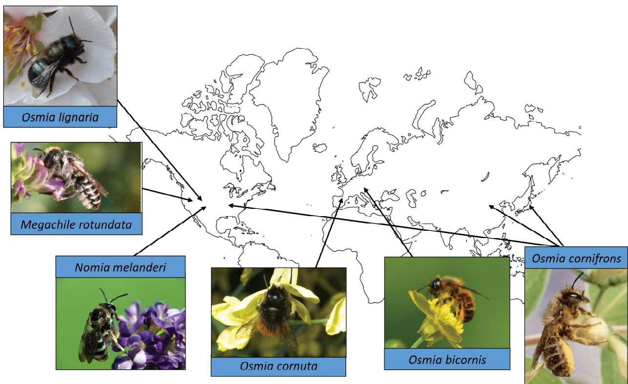
Fig. 1. Solitary bee species commercially available in different parts of the world. Photo credits: Osmia lignaria (Derek Artz), Megachile rotundata (Theresa Pitts-Singer), Nomia melanderi (James Cane), Osmia cornuta (Fabrizio Santi), Osmia bicornis (Laura Bortolotti), Osmia cornifrons (Suzanne Batra).
