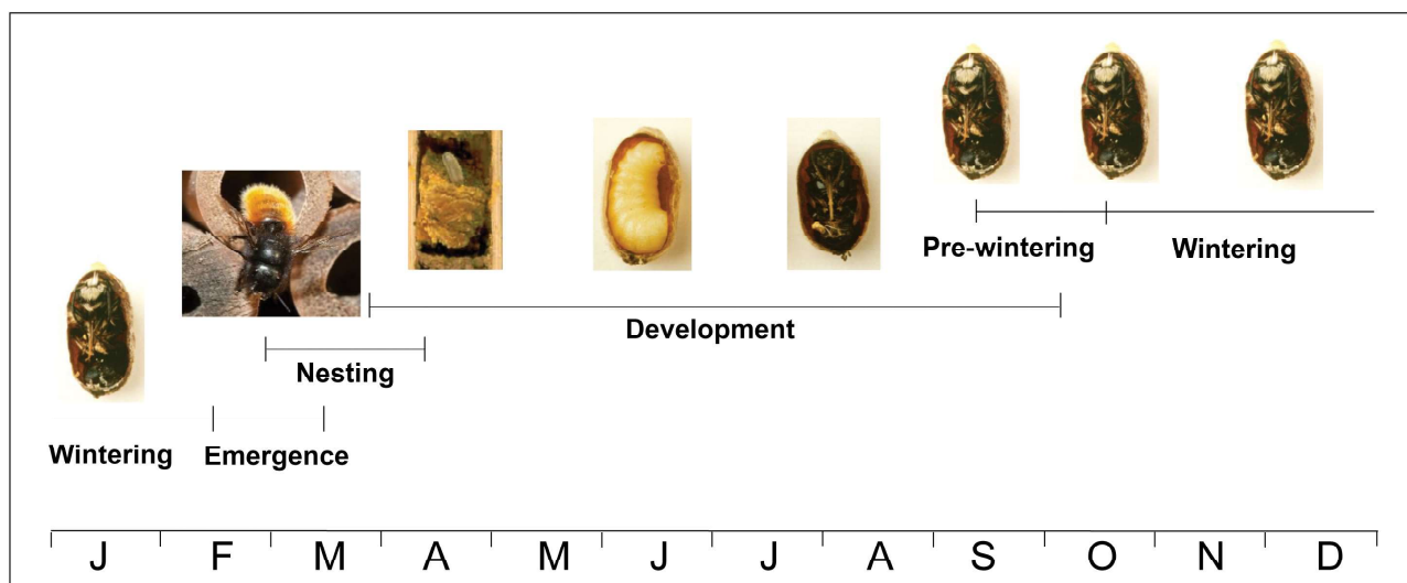
Fig. 3. Life cycle of Osmia spp. Photo credits: egg (USDA), prepupa (USDA), pupa (USDA), cocooned adult (USDA), emerged adult (Serena Magagnoli).
