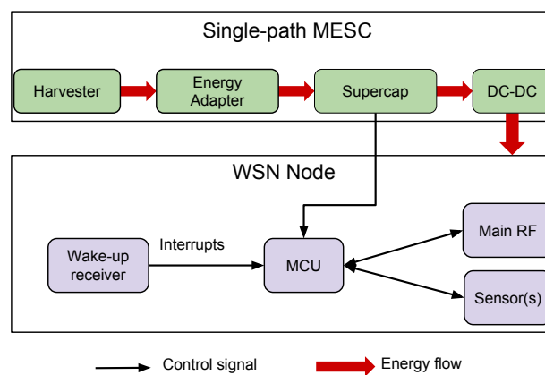
Figure 5. Hardware architecture of a WSN node using the Multiple Energy Source Converter (MESC) architecture and a WuRx. UPMA, Unified Radio Power Management Architecture.
