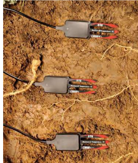
Plate 2 Decagon probes installed in soil, placed at three different depths to measure volumetric soil moisture, soil temperature and electrical conductivity
