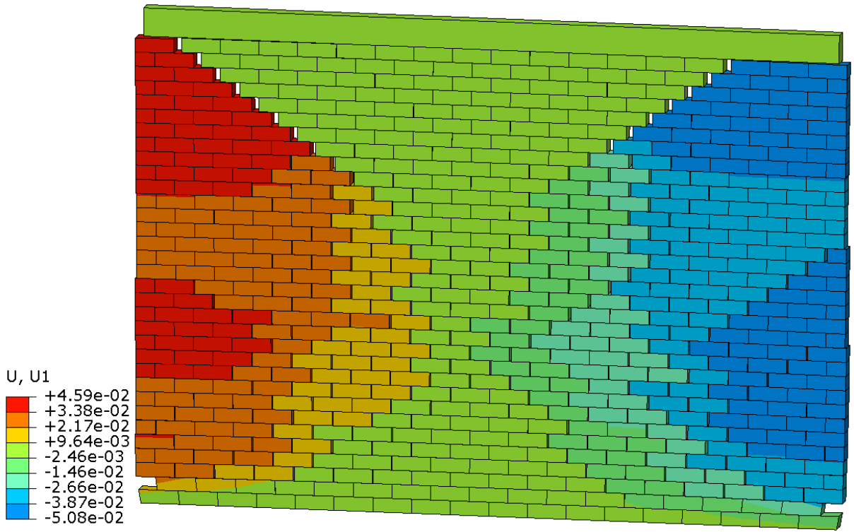
Fig. 16 – Thick wall (COMP-6) crack pattern comparison: photo of the cracked wall (a) and deformed horizontal displacement contour plot (b) in meters.
