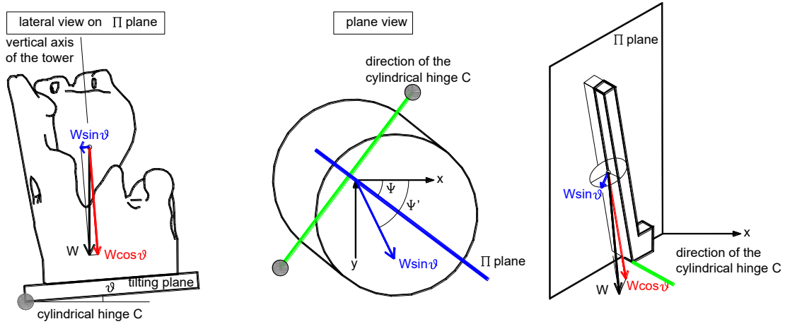
Fig. 7 –Limit analysis strategy for evaluating the collapse inclination of the 3D structure.
