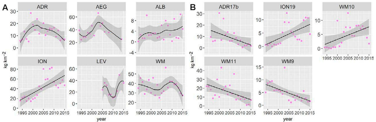
Fig. 7. – Chelidonichthys cuculus . Mean and 95% confidence intervals of the MEDITS relative biomass index ( \text{kg km}^{-2} ) in the Mediterranean ecoregions (A) and geographical sub-areas (GSAs, B) where a significant linear trend was found. GSA codes: 10, southern and central Tyrrhenian Sea; 11, Sardinia; 17b, NE Adriatic Sea; 19, western Ionian Sea; 9, Ligurian Sea and northern Tyrrhenian Sea.
