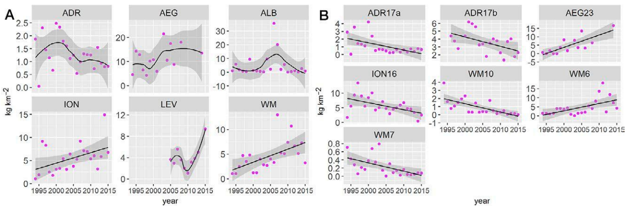
Fig. 12. – Chelidonicichthys lastoviza . Mean and 95% confidence intervals of the MEDITS relative biomass index (kg km -2 ) in the Mediterranean ecoregions (A) and geographical sub-areas (GSAs, B) where a significant linear trend was found. GSA codes: 10, southern and central Tyrrhenian Sea; 16, south of Sicily; 17a, NW Adriatic Sea; 17b, NE Adriatic Sea; 23, Crete; 6, northern Spain; 7, Gulf of Lions.
