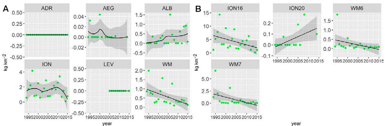
Fig. 8. – Chelidonichthys obscurus . Mean and 95% confidence intervals of the MEDITS relative biomass index ( \text{kg km}^{-2} ) in the Mediterranean ecoregions (A) and geographical sub-areas (GSAs, B) where a significant linear trend was found. GSA codes: 16, south of Sicily; 20, eastern Ionian Sea; 6, northern Spain; 7, Gulf of Lions.
