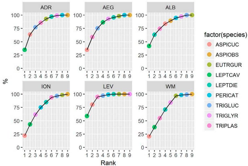
Fig. 3. – Species rank-accumulation (k-dominance) curves of gurnards in the six Mediterranean ecoregions. ADR, Adriatic Sea; ALB, Alboran Sea; AEG, Aegean Sea; ION, Ionian Sea; LEV, Levantine Sea; WM, western Mediterranean. Species code as in Figure 2.
