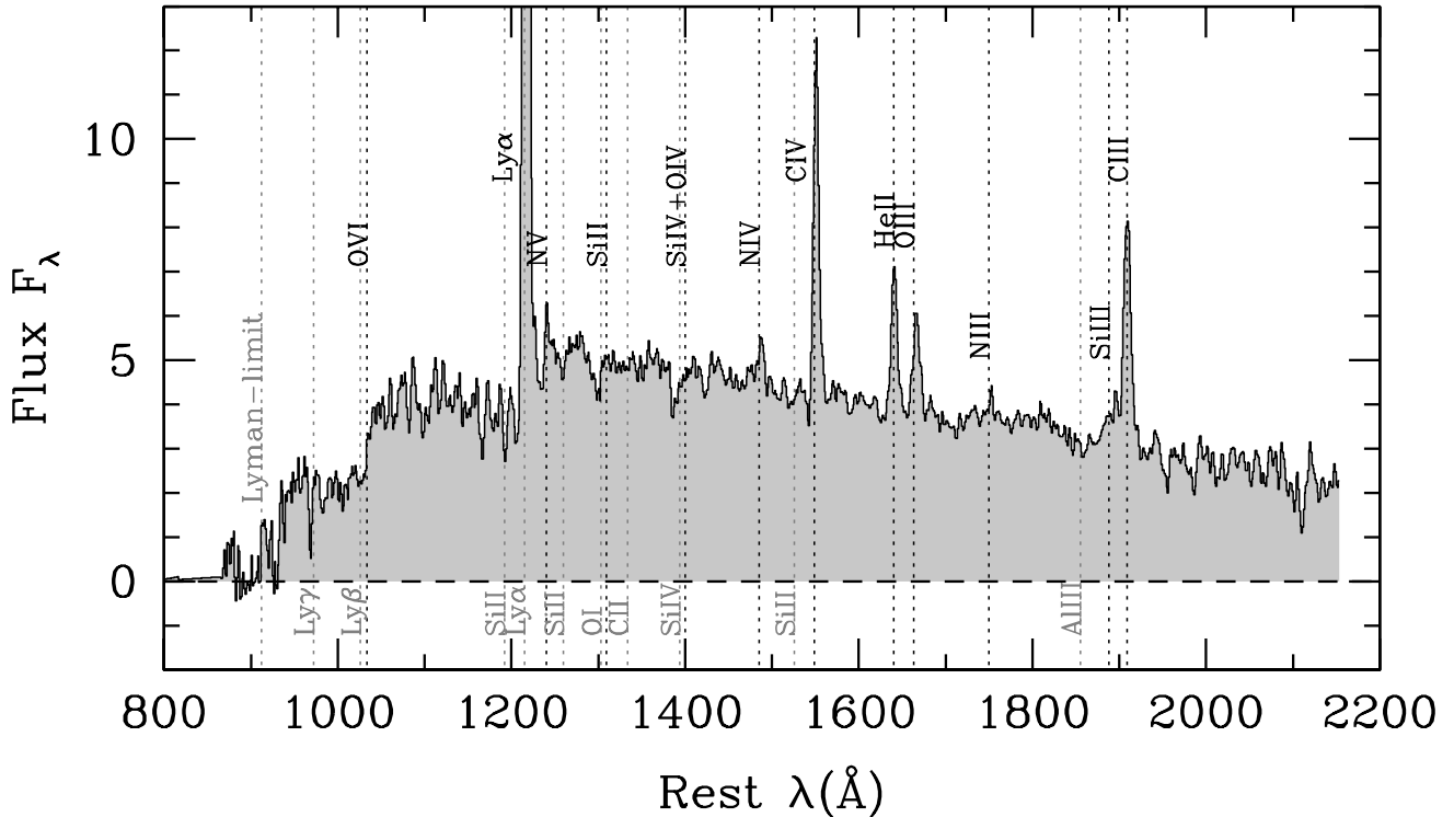
Fig. 5. Composite spectrum of 16 CIII]- \lambda 1908 emitters identified in the VUDS survey at 2 < z < 3.8 , where CIII] is detected in emission with S/N > 5 and EW(\text{CIII])} > 20 \text{ \AA} . The main emission lines associated with CIII]- \lambda 1908 emission can be identified as Ly \alpha , NV- \lambda 1240, NIV]- \lambda 1485, CIV- \lambda 1549, HeII- \lambda 1640, OIII]- \lambda 1663, NIII]- \lambda 1750, and SiIII]- \lambda 1888.
