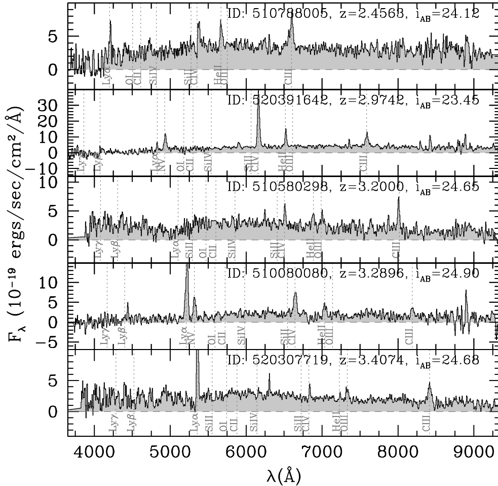
Fig. 1. Example VUDS spectra of CIII]1908 emitters with very strong \text{EW}(\text{CIII])} \geq 20 Å. The spectra of strong CIII] emitters are highly diverse: they include strong Ly- \alpha emission as well as weak Ly- \alpha emission (ID:510788005 and ID:510580298).
