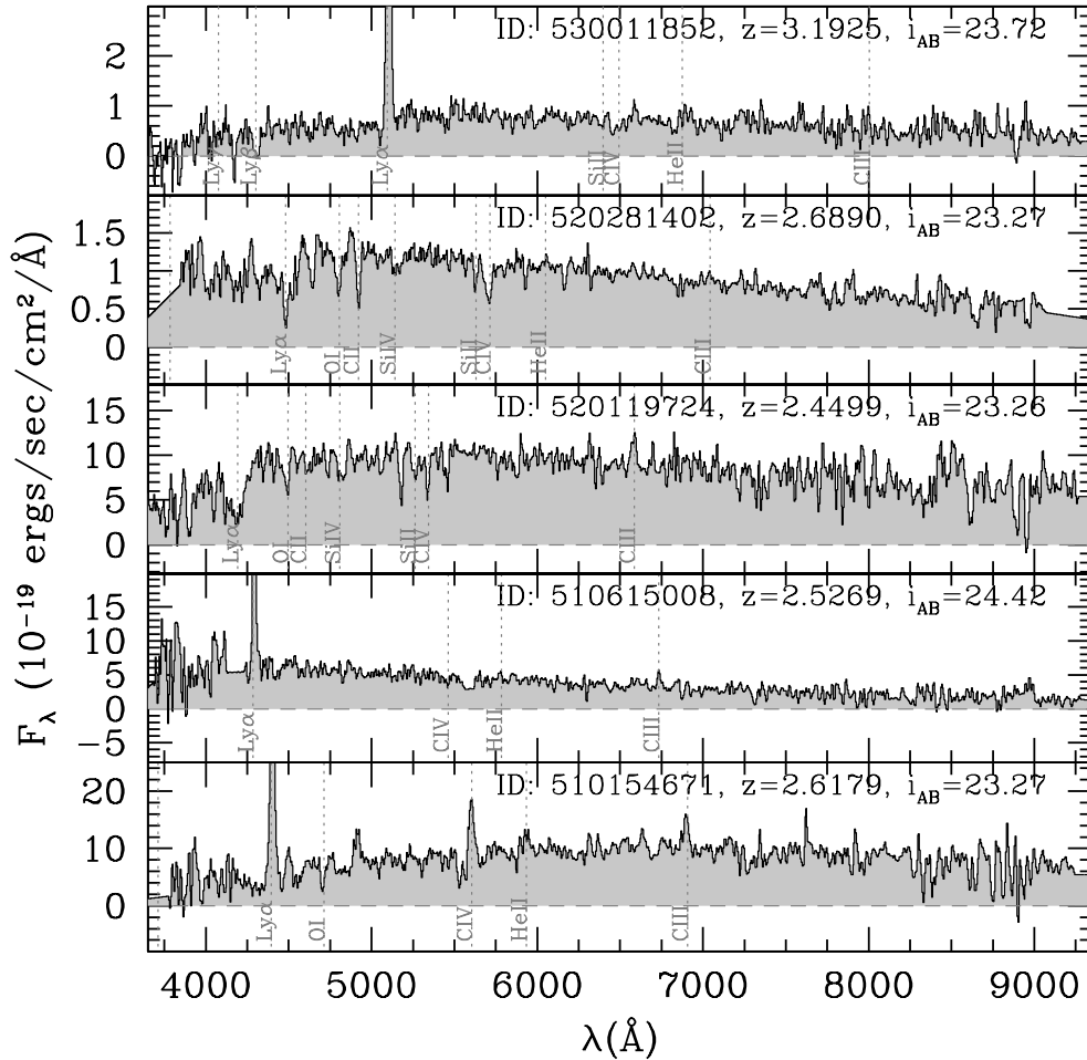
Fig. 3. Example VUDS spectra of weak CIII]1908 emitters with 0 < \text{EW}(\text{CIII])} < 5 Å.
