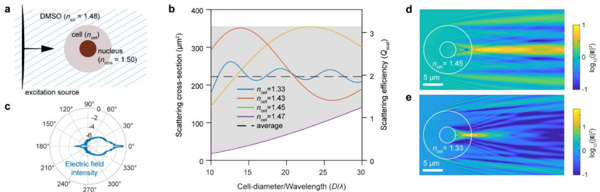
Figure 4. a. Schematic illustration of a cell in DMSO, modelled as a sphere with a core-shell structure. The nucleus is one third the size of the cell ( D = 12 \mu\text{m} , nucleus = 4 \mu\text{m} ). b. Scattering cross-section and scattering efficiency (cross-section/geometrical area) of the cell calculated by 3D Finite-Difference Time-Domain (FDTD) simulations. The cross-section is shown as a function of D/\lambda for different cell refractive indices (colored solid lines). On average, the cross-section is 220 \mu\text{m}^2 (dashed line). The grey region indicates the range of possible values due to
