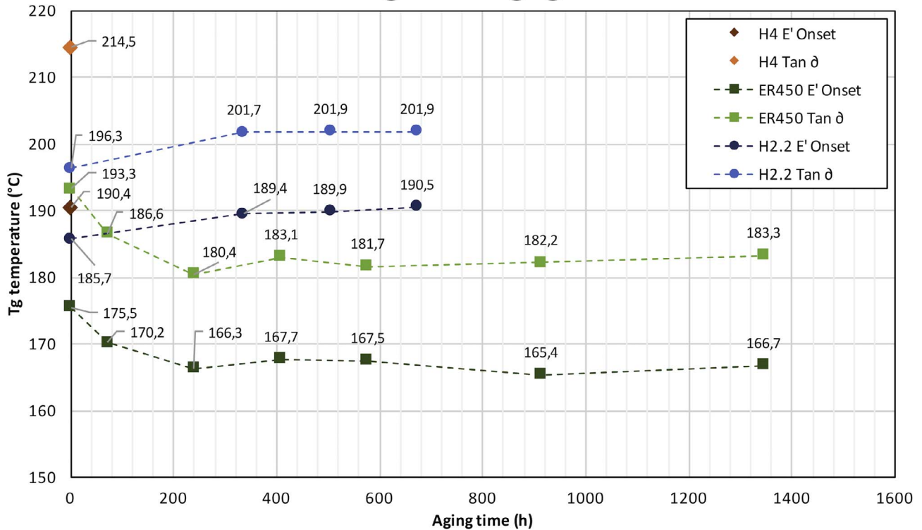
Fig. 12. Glass transition, evaluated both E' onset ( T_{\alpha_{E'}} , extrapolation of the first storage modulus E' loss) and tan \delta (taken as the peak of the damping factor), displayed as a function of aging time at 180 °C.
