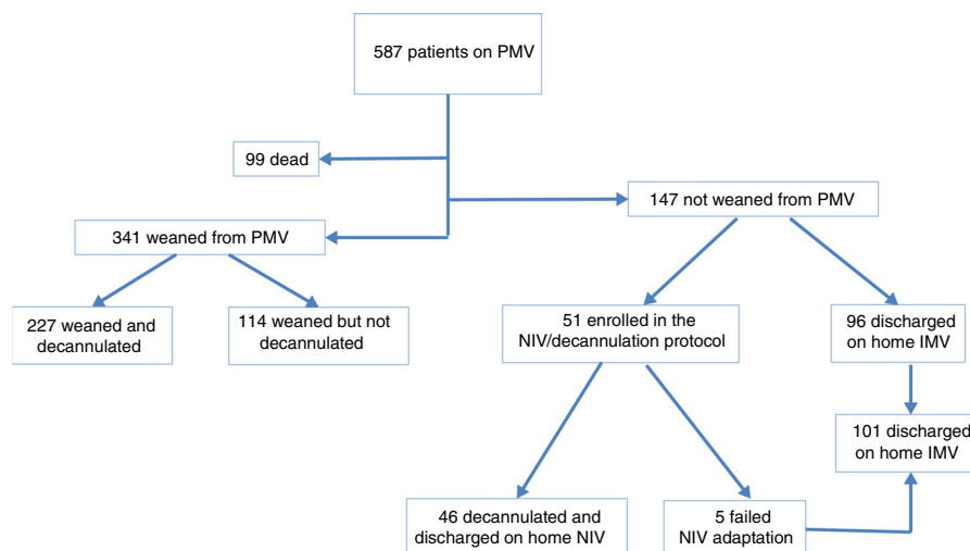
Figure 1 Population in study. IMV, invasive mechanical ventilation; NIV, non invasive ventilation; PMV, prolonged mechanical ventilation; VAIs, ventilator-assisted individuals.
