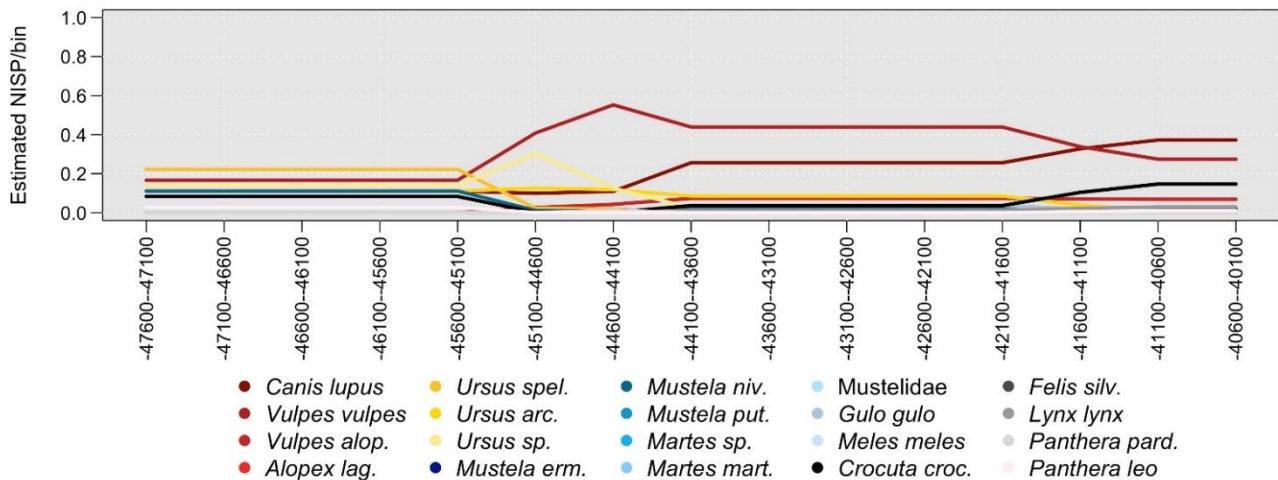
Fig. 10. Estimated diachronic relative frequency of each carnivore taxon at Grotta di Fumane, based on aoristic sums computed for 500-year temporal bins. Horizontal axis indicates dates cal. BP.
