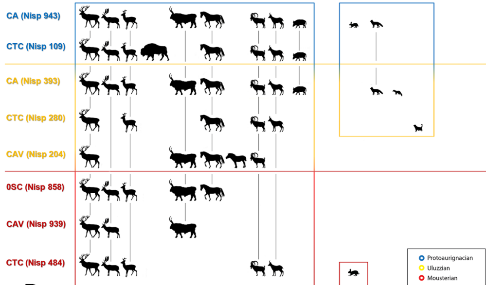
Fig. 13. Comparative summary of diachronic trends concerning the presence of taxa whose bones bear cut-marks, percussion marks and/or evidence of combustion. A) Northern Italy. RF = Grotta di Fumane; RB = Riparo del Broion; GSB = Grotta di San Bernardino; RS = Grotta del Rio Secco. B) Southern Italy. CAV = Grotta del Cavallo; OSC = Riparo l'Oscurusciuto; CTC = Grotta di Castelcivita; CA = Grotta della Cala. Colors of temporal phases: Protoaurignacian = blue; Uluzzian = yellow; Late Mousterian = red (for interpreting the color coding in the figure legend the reader is referred to the Web version of this article).
