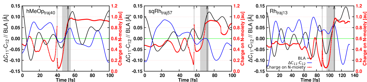
Figure 4. Selected examples show the evolution of BLA (bond-length alternation), C_{11}-C_{12} and charge on C_{12} ---N fragment during the simulation in the three rhodopsins, ( \Delta C_{11}-C_{12} represents the deviation of C_{11}-C_{12} from 1.45Å), gray-shaded areas denote the time span in which the WF changes from CT to covalent after a hopping event, vertical dashed and solid arrows show the hopping and decision times, respectively.
