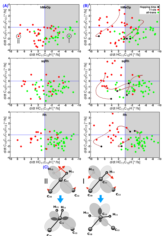
Figure 3. Distribution of the hopping (A) and decision (B) events as a function of the magnitude and directionality of the HCC and CCCC velocities. Green and red circles show trajectories that lead to the photoproduct or reactant formation, respectively. The brown lines show some examples for the change of dihedral angle directionality during the period between the hopping event (black circles) and the decision event. C. Schematic representation of the in-phase (diagram I) and out-of-phase (diagram II) \pi -overlap across the C_{11} - C_{12} bond. Notice that I would
