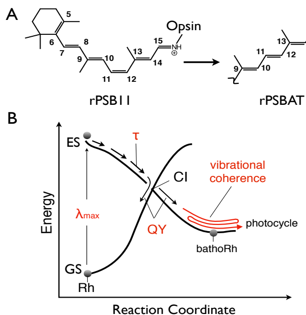
Scheme 1. Animal rhodopsin isomerization. A. -C_{11}-C_{12}- double-bond isomerization in bovine rhodopsin. B. Schematic representation of the ES and GS energy profiles controlling the ultrafast photoisomerization of bovine rhodopsin. The critical properties relevant to the present work are indicated in red.
