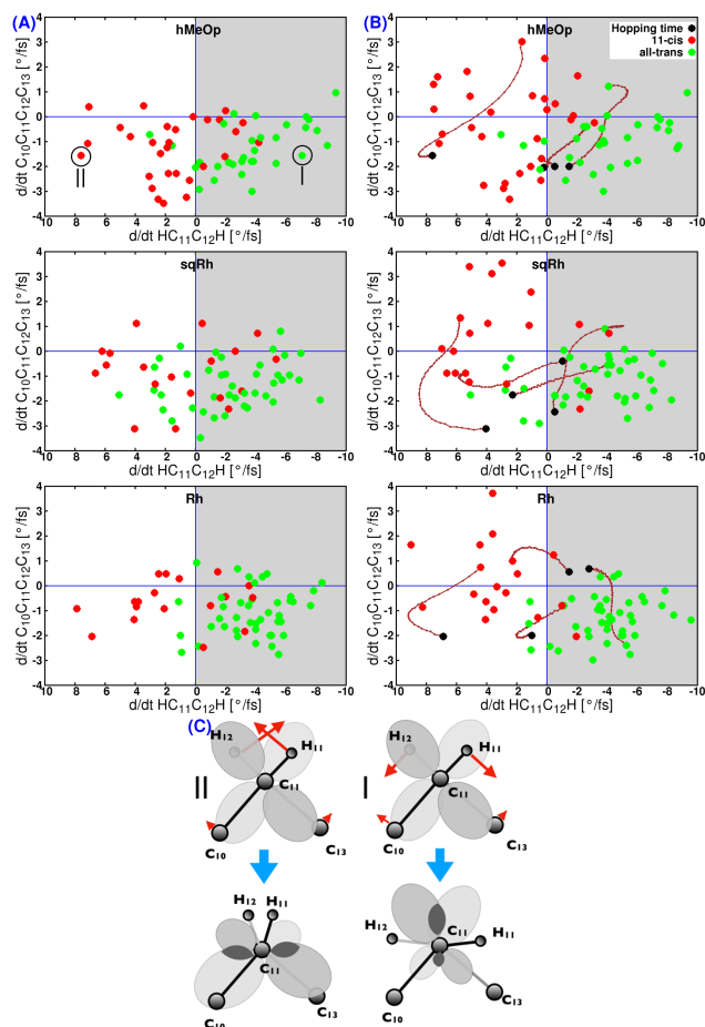
Figure 3. Distribution of the hopping (A) and decision (B) events as a function of the magnitude and directionality of the HCCCH and CCCC velocities. Green and red circles show trajectories that lead to the photoproduct or reactant formation, respectively. The brown lines show some examples for the change of dihedral angle directionality during the period between the hopping event (black circles) and the decision event. C. Schematic representation of the in-phase (diagram I) and out-of-phase (diagram II) \pi -overlap across the \text{C}_{11} - \text{C}_{12} bond. Notice that I would
