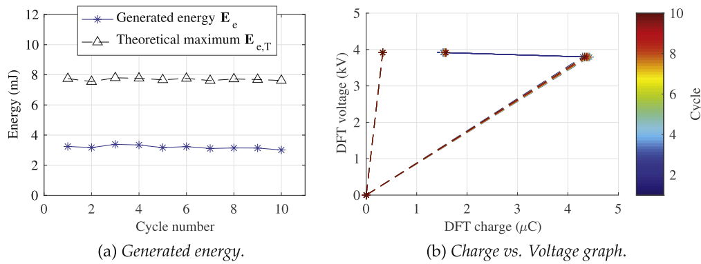
Figure 14. Results of the repeatability test. V_{in} = 4 \text{ kV} , Q_{out} = 16 \text{ cm}^3 \text{ s}^{-1} , Q_{in} = 72 \text{ cm}^3 \text{ s}^{-1} . Figure 14(a) shows a substantially constant energy generated in consecutive cycles. In figure 14(b) the main elements of the graphical representation of the generated energy are represented for each cycle.
