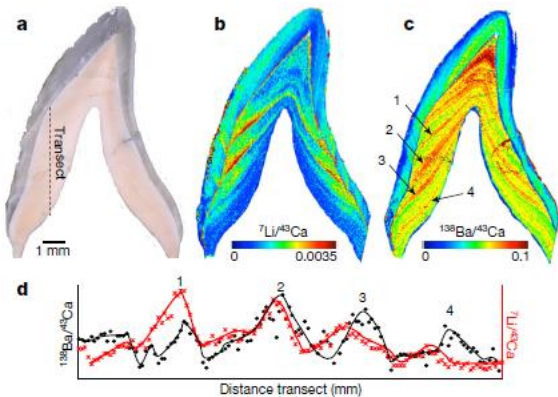
Fig. 3 | Elemental mapping of StS 51A africanus canine. a, Micrograph (10 \times magnification) of StS 51B permanent lower canine. b, c, Associated elemental mapping of 7 Li/ 43 Ca (b) and 138 Ba/ 43 Ca (c). Permanent canine teeth develop only a few months after birth, with completion of the crown between three and four years of age 18 . d, Comparison of the temporal periodicity of Ba/Ca (black line and diamonds) and Li/Ca (red line and crosses) accentuated lines (labelled 1, 2, 3 and 4), along the transect illustrated in a. Li/Ca recurrence shows a slight temporal offset compared to Ba/Ca periodicity.
