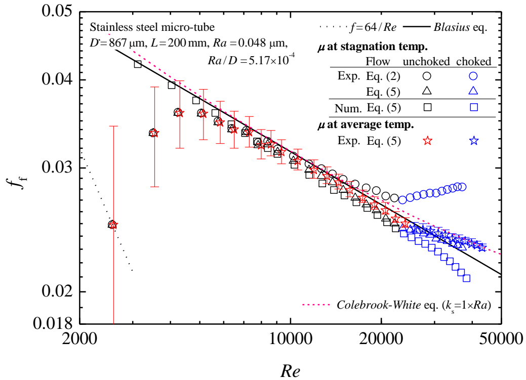
Fig.1 Fanning friction factor as a function of Re
