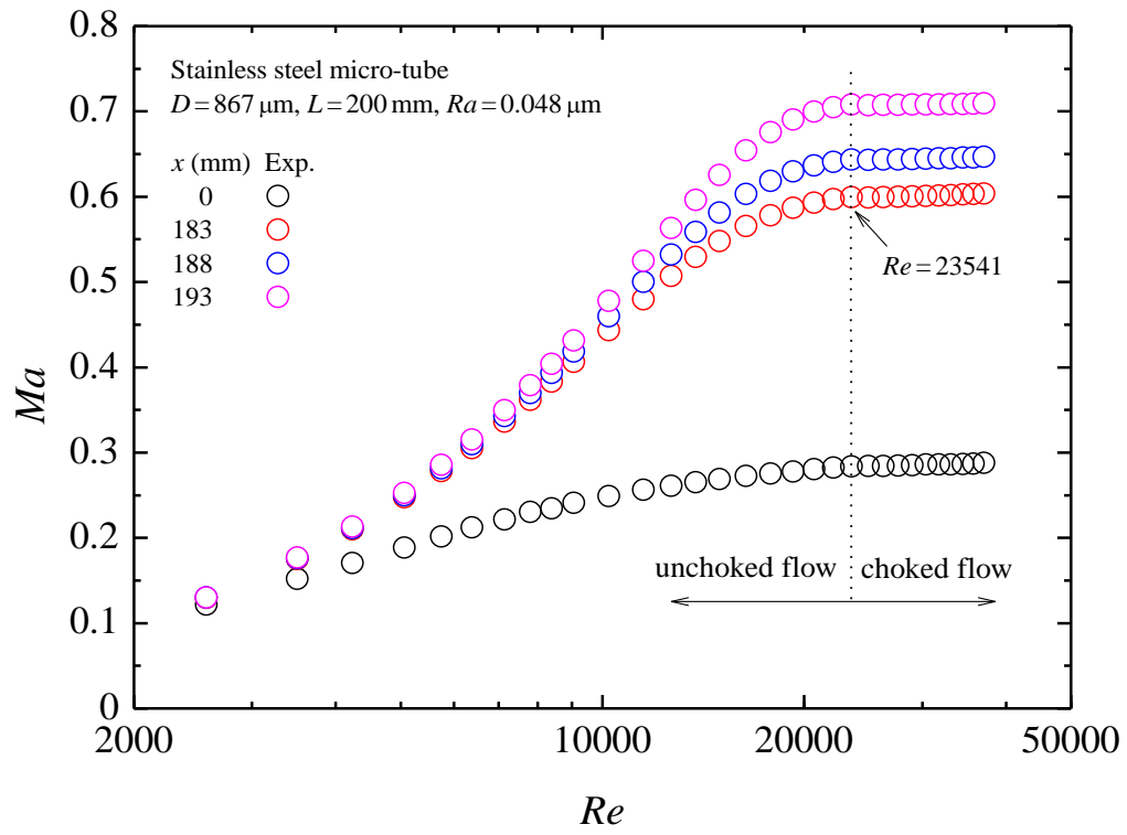
Fig. 2 Mach number as a function of Re
