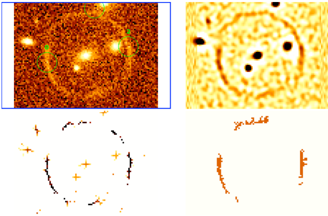
Fig. 1. GAHEC IRAP. From top-left to bottom right: 1) a simulated arc extracted from the strong lensing challenge in which an tuned Arcfinder selects 3 candidates (green circles), 2) the smoothed image on which pixel wise elongation is computed, 3) the resulting elongated pixels after threshold, 4) the set of pixels selected for the computation of arc candidate properties.
