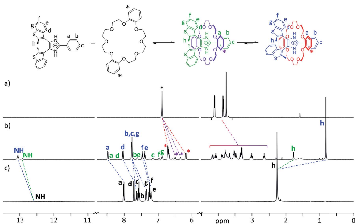
Fig. 2 ^1\text{H} NMR spectra of (a) DB24C8, (b) [2]pseudorotaxane [1_o\text{-H-CD}24\text{C8}]\text{BF}_4 , and (c) [1_o\text{-H}]\text{BF}_4 . Corresponding peaks are matched by dashed lines; the axle peaks and the aromatic peaks of the macrocycle are labelled using colours matching the accompanying reaction scheme.
