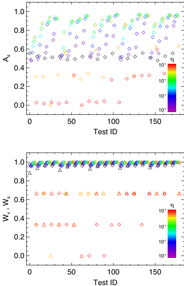
Figure 5. Accuracy parameters A_s (top panel), W_v and W_s (diamonds and triangles, respectively, bottom panel) in tests with different combinations of learning rate, batch size and number of epochs ( \eta , N_b , N_e ). The three parameters can take the following values: \eta = [10^{-6}, 5 \times 10^{-6}, 10^{-5}, 3 \times 10^{-5}, 5 \times 10^{-5}, 7 \times 10^{-5}, 10^{-4}, 5 \times 10^{-4}, 10^{-3}] , N_b = [15, 30, 50, 64, 100] , N_e = [10, 20, 50, 100] . Each combination ( \eta , N_b , N_e ) is characterized by a different TestID (an integer number between 1 and 180). Colours (in logarithmic scale) represent the parameter \eta .
