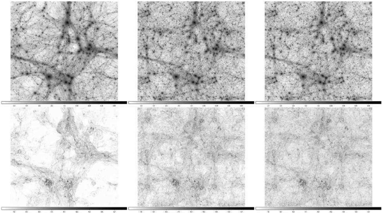
Figure 2. Progression of our sky model for a 16 \times 16 \text{ deg}^2 area, as a function of the maximum redshift of integration: z = 0.04 (first panel), z = 0.2 (second) and z = 0.5 (third). The top row shows the projected gas density while the second row shows the total radio emission, at the frequency of ASKAP.
