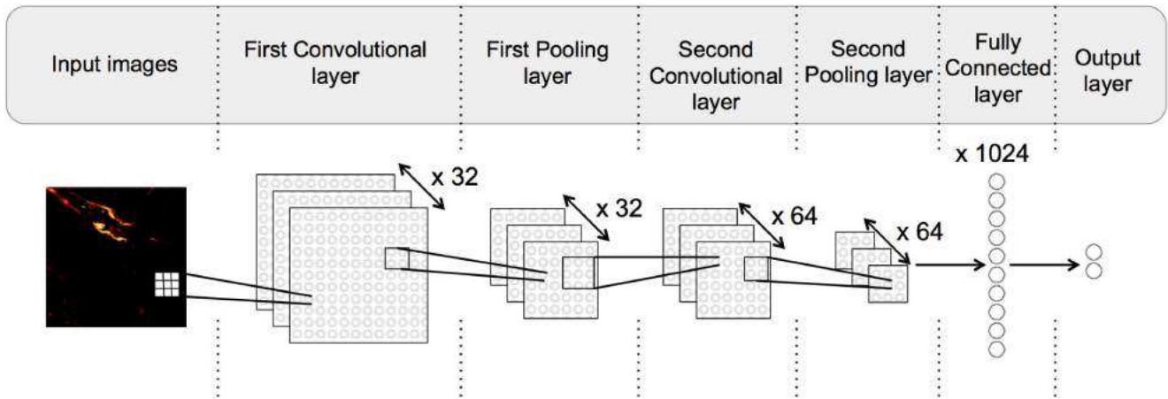
Figure 1. The COSMODEEP CNN architecture, accounting from one input, five hidden and one output layers.
