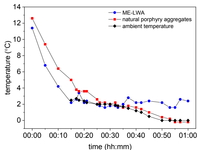
Figure 15. Development of temperature as a function of time using the infrared thermometer.
