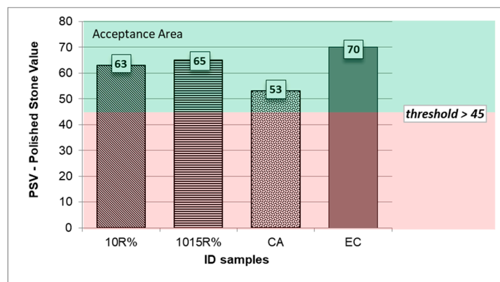
Figure 13. Histogram of average Polished Stone Values for samples 10%R, 1015%R and CA compared with PSVs of expanded clay and acceptance threshold values (green area) from common Italian technical specifications. (Note: in the figure PSVs are \times 100 .)
