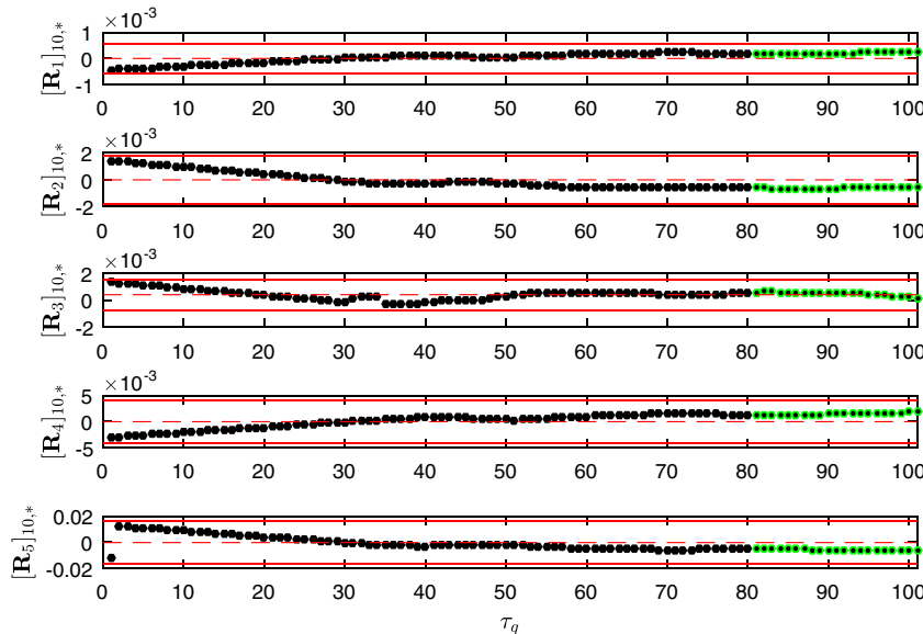
FIGURE 6 Training and validation stages: samples of the residual matrix at Node 10 for the first five vibration modes. The black dots correspond to the long-term scale temporal points of the estimation set \mathcal{T}_e(\tau) , and the green dots to the ones of the validation set \mathcal{T}_v(\tau) . The red dashed line corresponds to the mean value \mu of the estimation samples (e.g., the black dots) and the red continuous lines to \mu \pm 3\sigma , where \sigma is the standard deviation of the estimation samples (Case study I)
