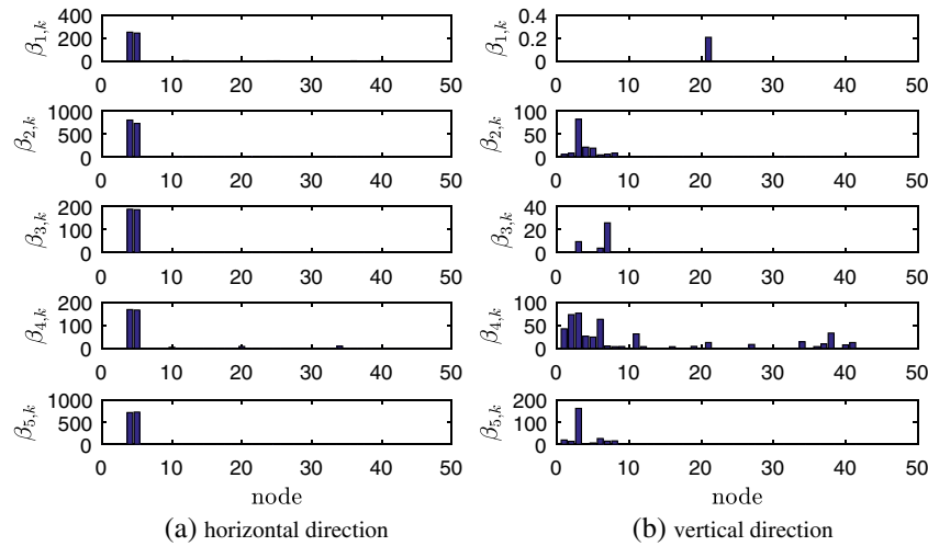
FIGURE 17 Diagnostics stage: damage index for 10% damage in Bar element 4 (Case study II).
