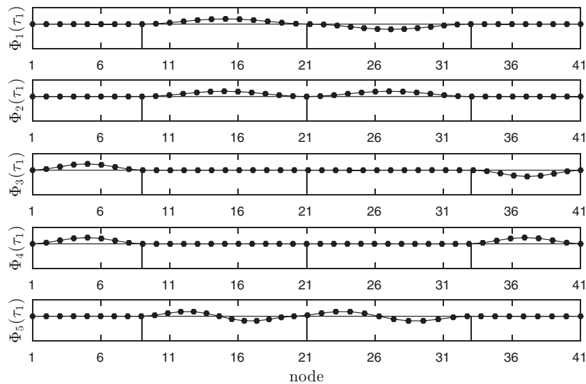
FIGURE 13 First five mode shapes of the bridge at \tau_1 (Case study II)
