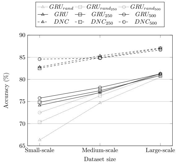
Figure 5: Average cross-domain with fine-tuning accuracy over the 12 source-target combinations of the 4 domains. The subscripts 250 and 500 represent the number of labelled target instances utilised for fine-tuning.
