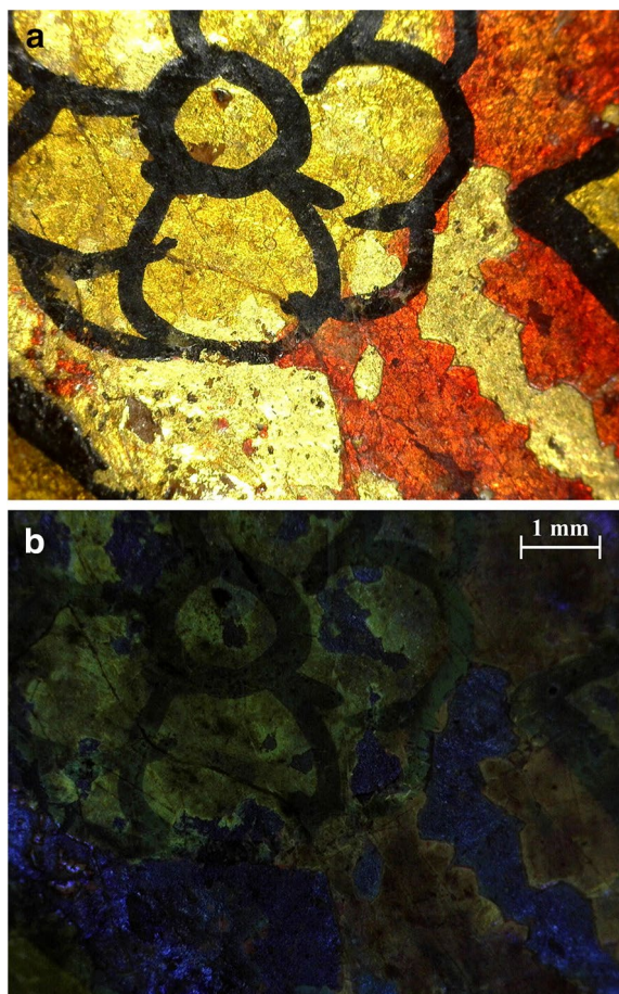
Fig. 4 Surface observation by digital microscope: floral pattern on incomplete red coloured background. Binding, right board. Images © Biblioteca Nazionale Marciana, Venice. a VIS light, \times 50 . b UV light, \times 50
