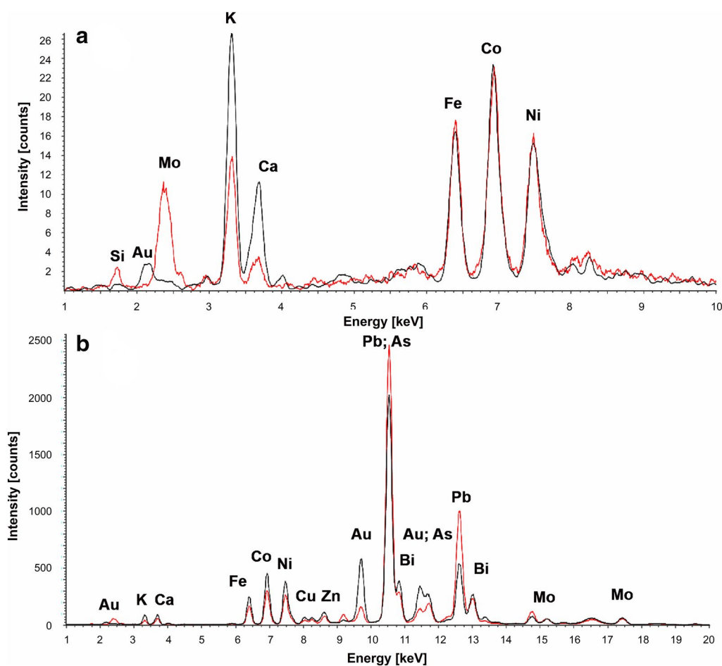
Fig. 9 XRF spectrum collected from the recto (black) and the verso (red) of sample 5_1869_BNM. a 50 kV, 700 \mu A and 1 mm collimator. b 12 kV, 110 \mu A and 0.2 collimator
