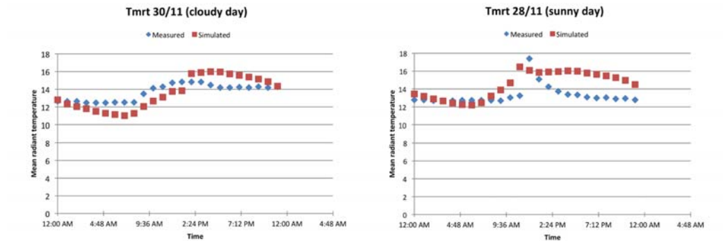
FIG. 6 Comparison between measured and simulated data of the MRT in the room during cloudy day (left) and sunny day (right)
