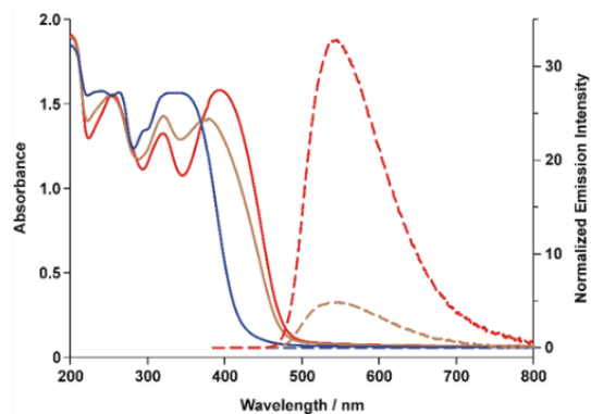
Figure 2. Absorption spectra (solid lines, left scale) and emission spectra (dashed lines, right scale; \lambda_{\text{ex}} = 380 \text{ nm} ) of a drop-casted film of 1 . The red lines are of 1-Z , the blue lines correspond to PSS 450 (> 90% 1-E ), and the brown lines depict the bands at PSS 360 .
