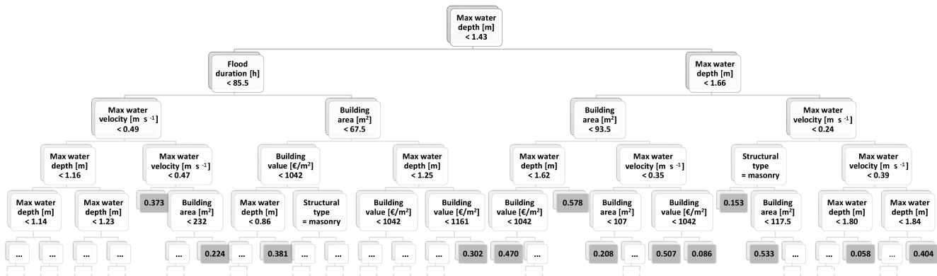
Figure B1. Example of a tree built with the RF algorithm on the basis of the Secchia dataset. White boxes represent splitting nodes, together with the indication of the splitting variable and its splitting value; grey boxes represent final nodes and the estimation of the relative building damages of that branch. The tree is cut off at an arbitrary level for the sake of clarity.
