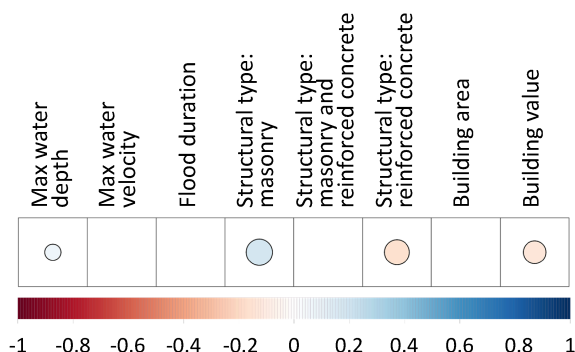
Figure 5. Spearman correlation between relative loss (buildings only) and predictive variables: maximum water depth, maximum water velocity, flood duration, structural type (masonry, masonry and reinforced concrete, or reinforced concrete), building area and building value per unit area. Empty boxes indicate statistically non-significant correlation coefficients at a 5 % significance level.
