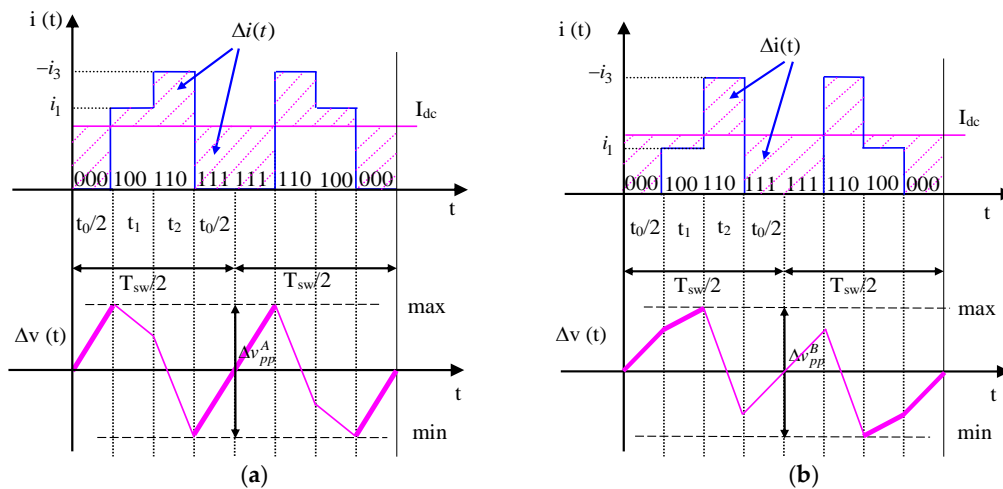
Figure 3. dc-link current and voltage ripple in one switching period: (a) Case A ( 0 \leq \vartheta \leq \pi/3, i_1 \geq I_{dc} ), (b) Case B ( 0 \leq \vartheta \leq \pi/3, i_1 < I_{dc} ).
