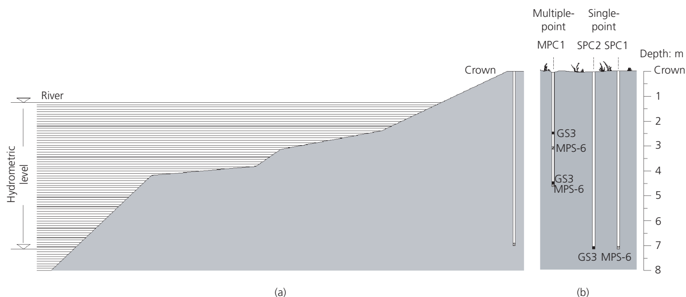
Figure 4. Scheme of the sensor installation: (a) cross-section with likely hydrometric levels and (b) longitudinal section
