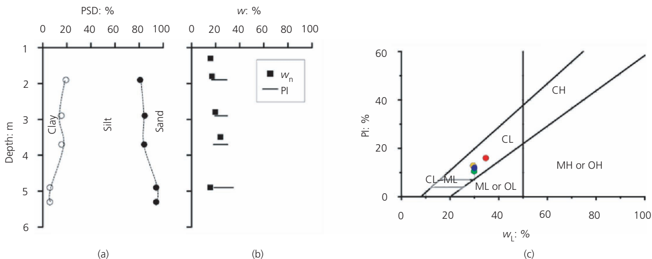
Figure 1. Soil classification at the installation site: (a) particle size distribution (PSD), (b) plasticity index and natural water content with depth and (c) Casagrande chart within the Unified Soil Classification System. C, clay; H, high plasticity; L, low plasticity; M, silt; O, organic
