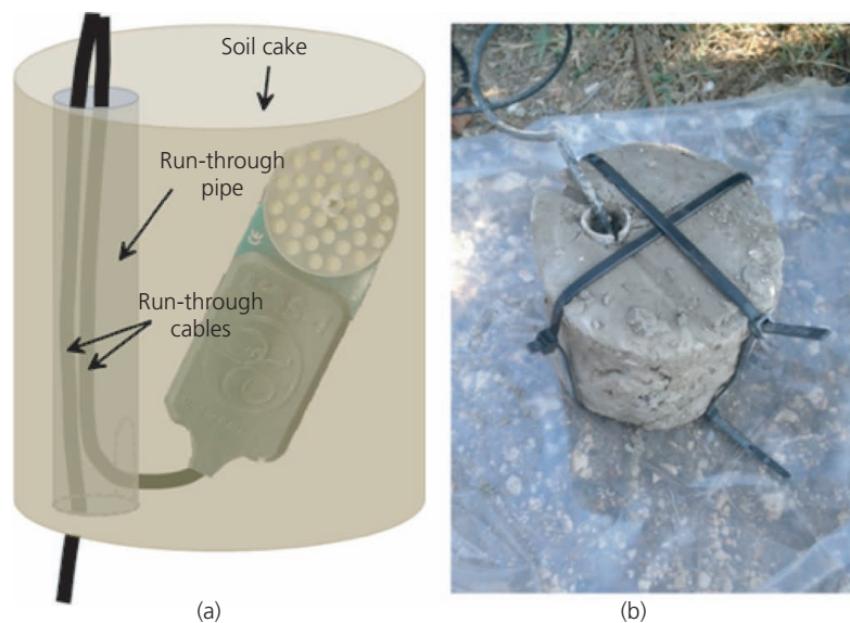
Figure 3. Schematic diagram of the ‘soil cake’ used for installing the suction sensor: (a) drawing and (b) photograph taken at the site prior to the installation
