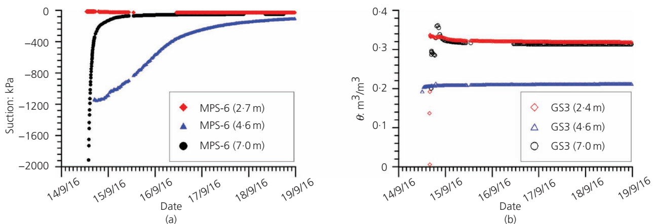
Figure 7. Monitoring data collected right after the sensor installation: (a) suction and (b) water content.
