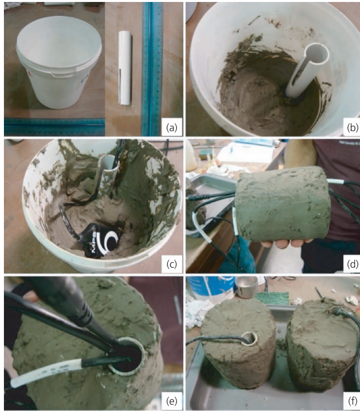
Figure 2. Phases of the laboratory preparation of the ‘soil cake’ used for installing the suction sensor: (a) tools required, (b) initial positioning of the tube, (c) placing of the MPS-6 sensor, (d) side view of sensor cables running through the cake, (e) top view, (f) cakes after curing
