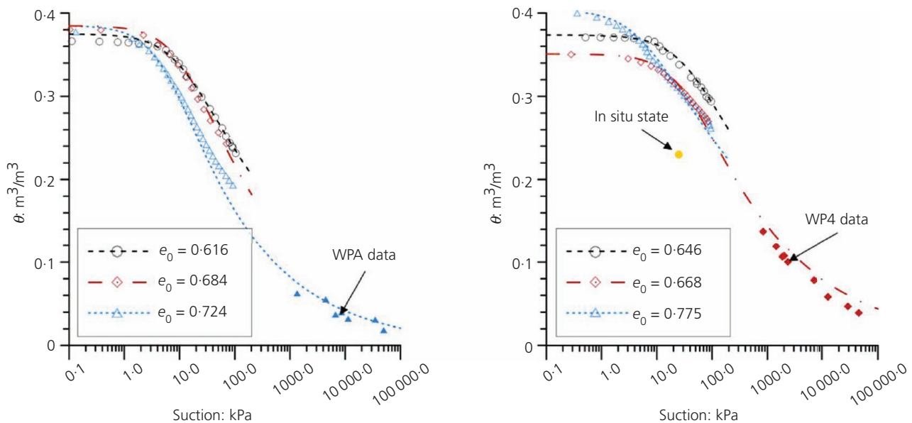
Figure 8. SWRCs for the main drying paths obtained by means of evaporation tests on remoulded soil sampled at (a) 2.8 and (b) 4.8 m depths from the surface. Field values (filled circle) at 4.5–4.6 m depth are plotted when equilibrium is fully reached (31 January 2017)
