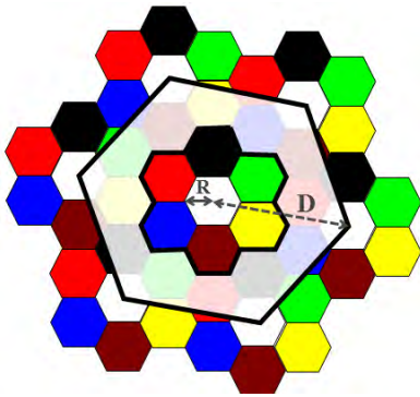
FIGURE 5. Hexagonal tessellation, omnidirectional case. The different colors account for the different radio resources assigned to the cells.
