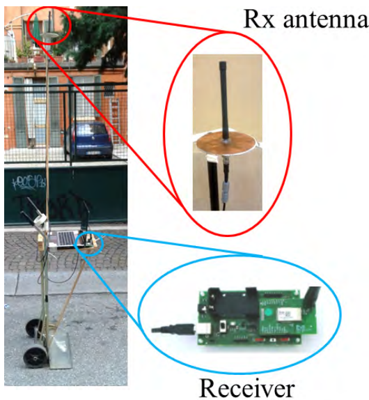
FIGURE 2. The receiver utilized in the measurement campaign carried out in Bologna, mounted on a mobile support.
